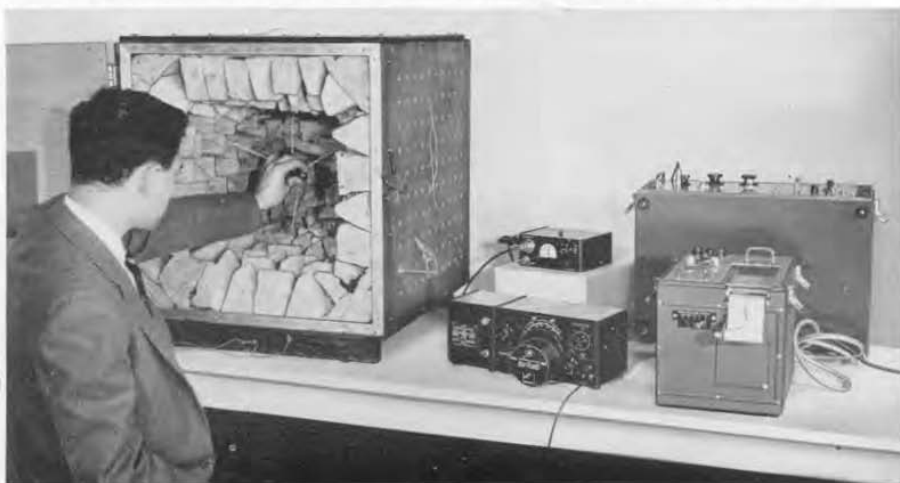
Figure 6. Setup for recording the frequency response of a small loudspeaker. The Type 1210-B Unit R-C Oscillator is swept over the frequency range of 2 kc to 20 kc by the Type 908-P1 Dial Drive. The output of the oscillator is amplified by a Type 1206-B Unit Amplifier which drives the loudspeaker. The loudspeaker is mounted in one wall of a small anechoic chamber. With the chamber completely closed, the output of the speaker is picked up by a condenser microphone, shown here as it is being put in place by the operator. This microphone is part of the Type 1551-P1 Condenser Microphone System. The signal from the microphone is amplified by the Sanborn Model 150-1400 Log Audio Preamplifier, shown in the upper right, and recorded on the Sanborn Model 151-100A Recorder Assembly, right front.
